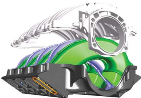
LSX R ™ 102mm Intake Manifold CAD
